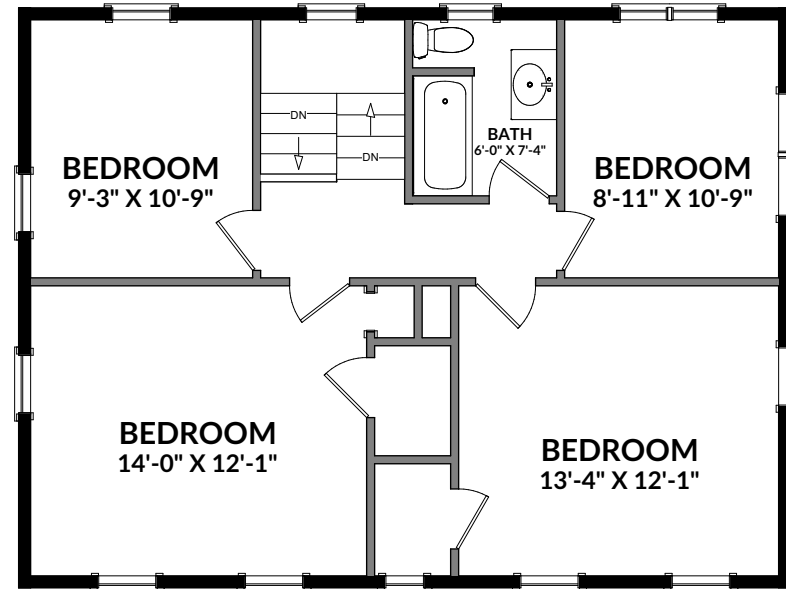
SECOND FLOOR
