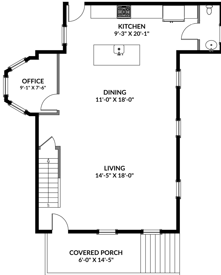
FIRST FLOOR
