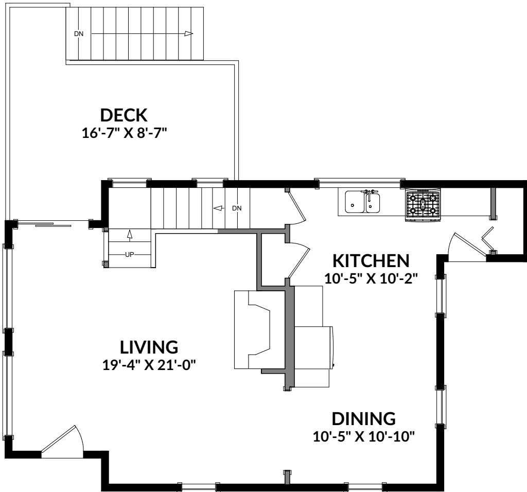
FIRST FLOOR
