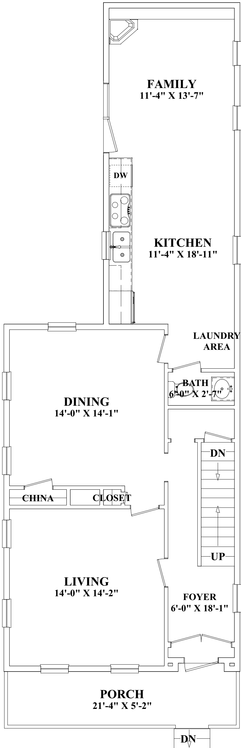
First Floor
