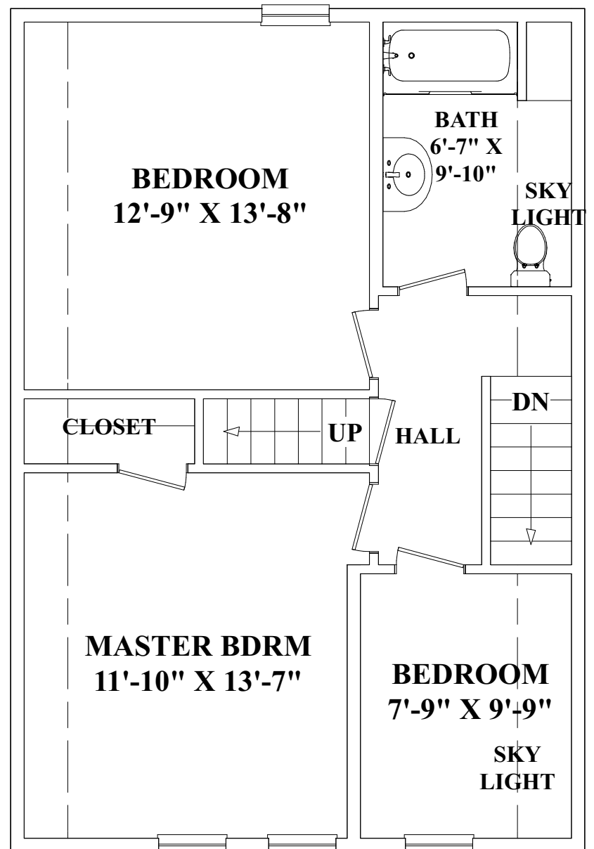
Second Floor
