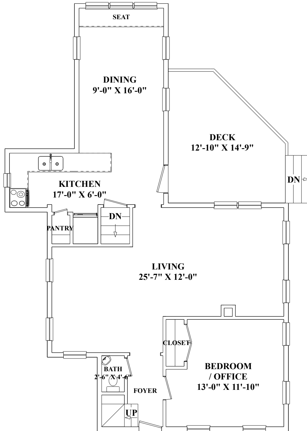
First Floor
