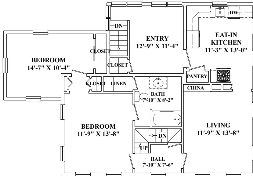
Second Floor
