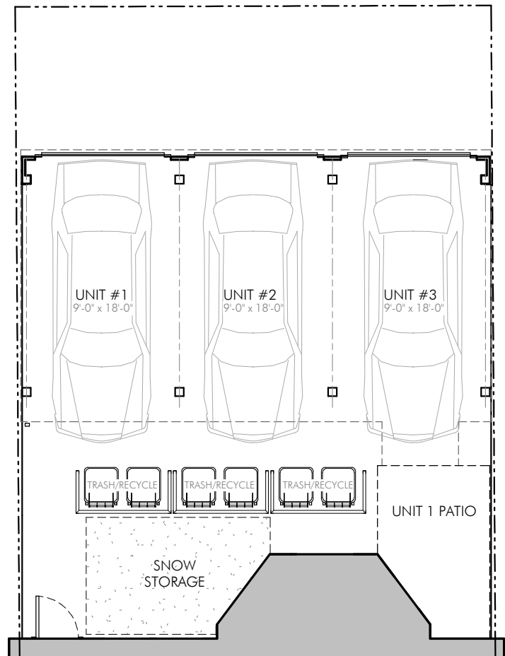
PARKING PLAN
