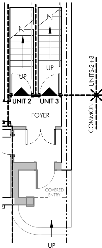
ENTRY PLAN
