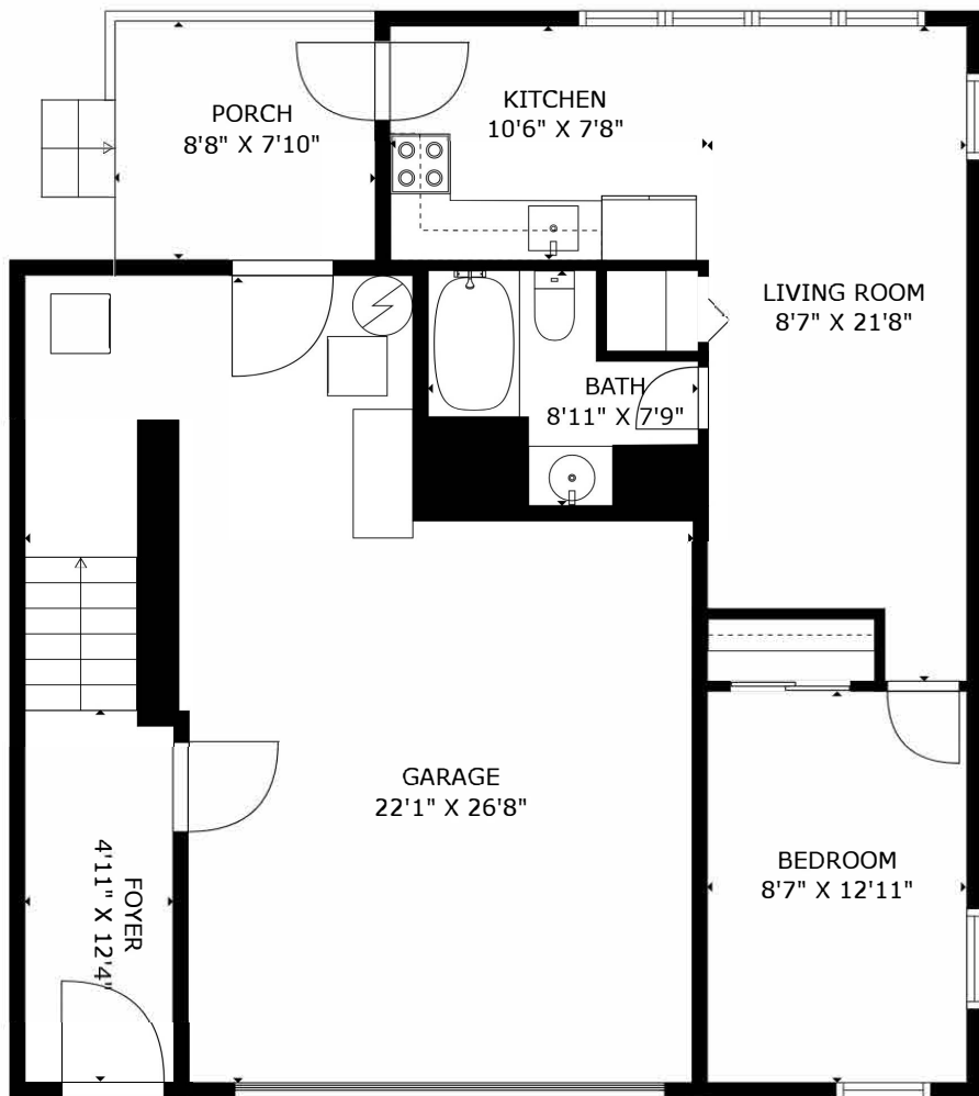
FLOOR 1
