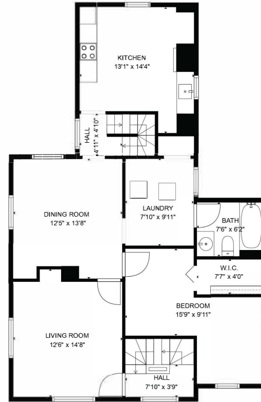
FLOOR 2 UNIT 2
