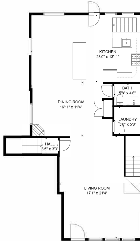
FLOOR 2
