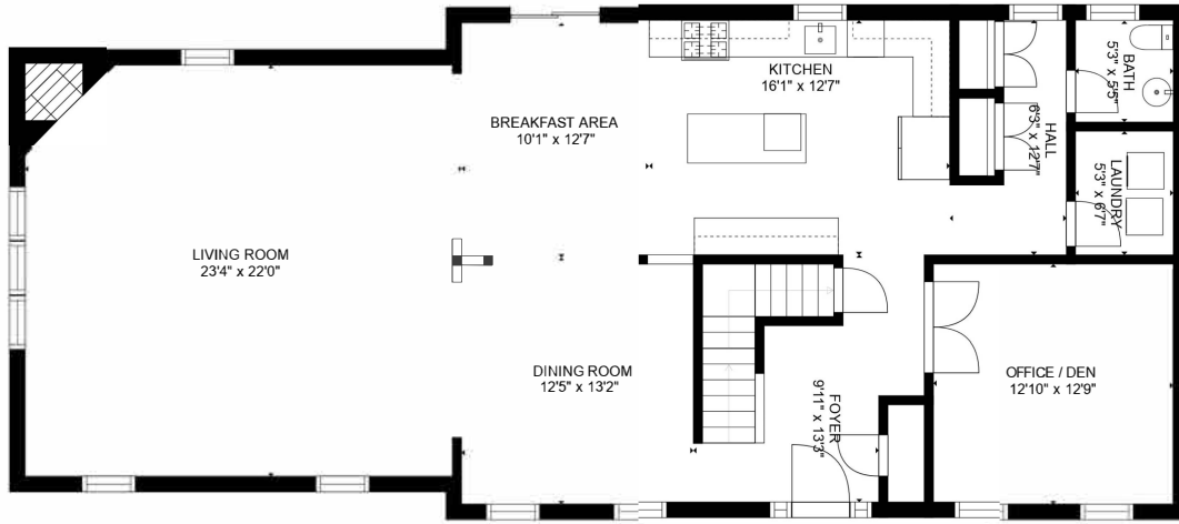
FLOOR 1
